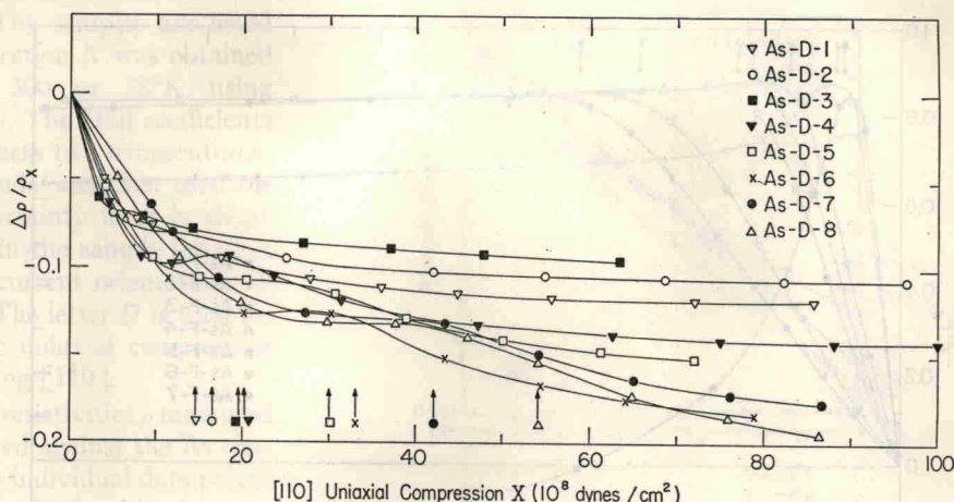
FIG. 4. Transverse piezoresistance as a function of [110] compressional stress with current along [110] at 1.2°K for As-doped germanium (arrangement D). The arrows indicate the saturation stress for undistorted parabolic bands.
