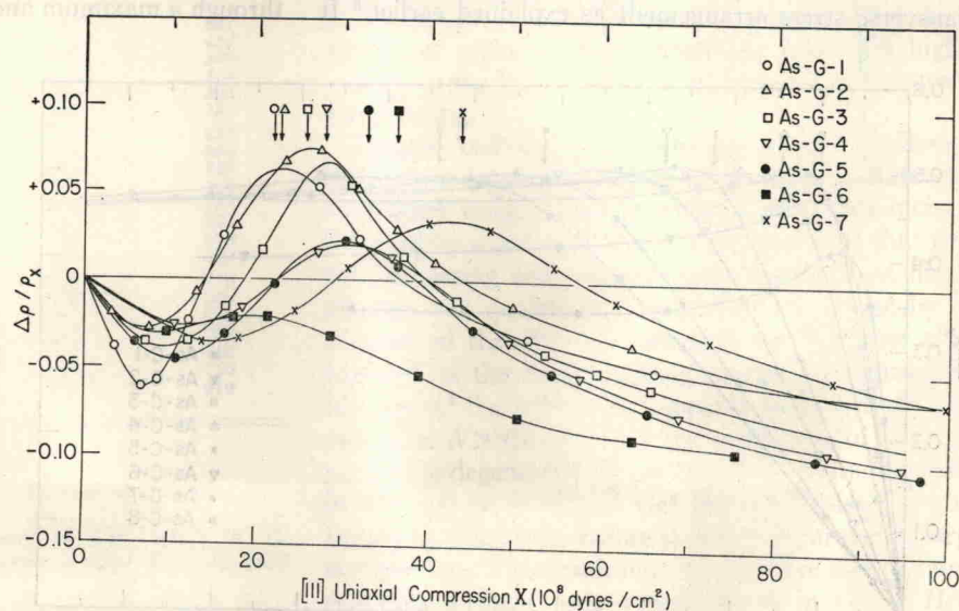
FIG. 5. Same as Fig. 4 for [111] compressional stress (arrangement G).
